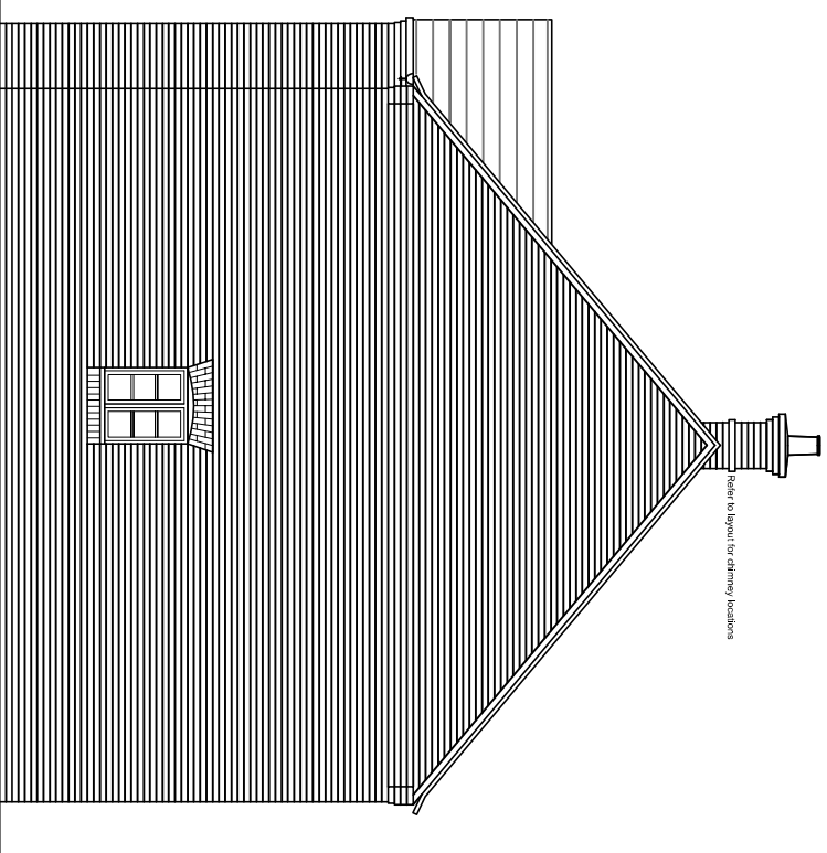
SIDE ELEVATION FORMAL TYPE E : P404
