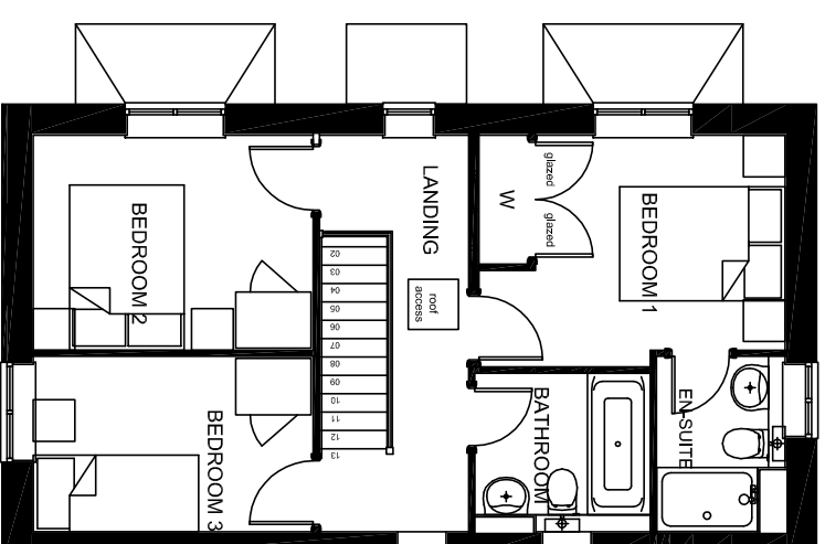
FIRST FLOOR PLOT : 100 TYPE B : P303
