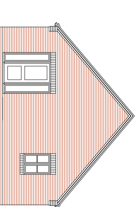
REAR ELEVATION FORMAL TYPE K : SB2
