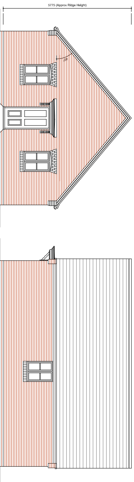
FRONT ELEVATION FORMAL TYPE K : SB2
