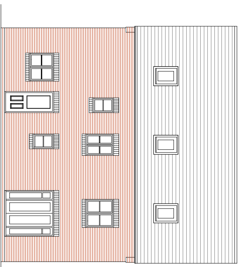
FRONT ELEVATION INFORMAL TYPE X : P504
