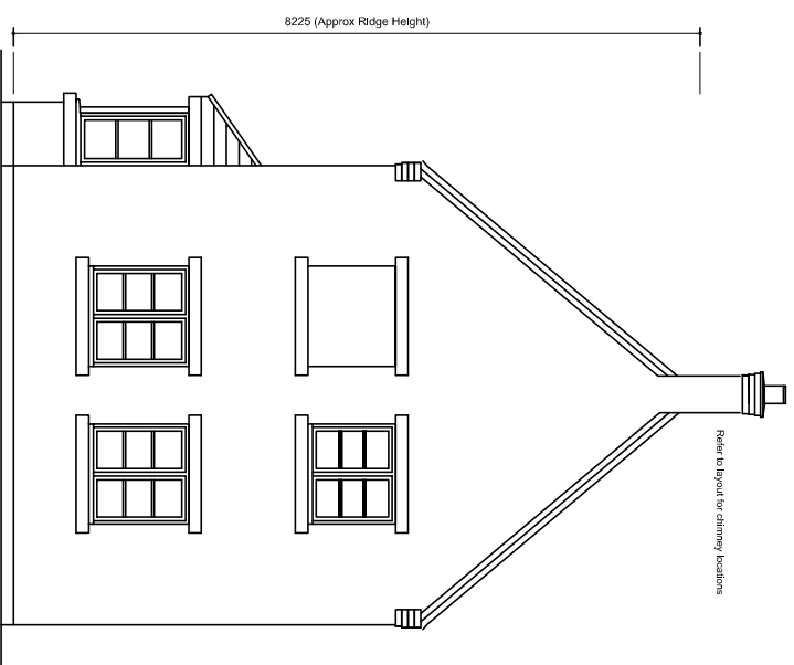
SIDE ELEVATION FORMAL PLOT : 100 TYPE B : P303
