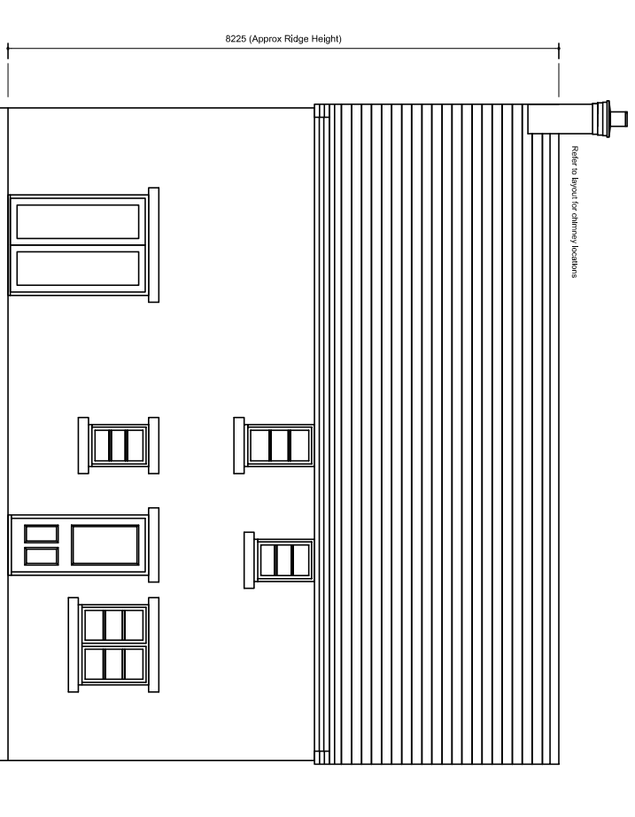
REAR ELEVATION FORMAL PLOT : 100 TYPE B : P303
