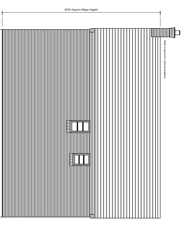
REAR ELEVATION INFORMAL PLOT : 70,91 TYPE B : P303
