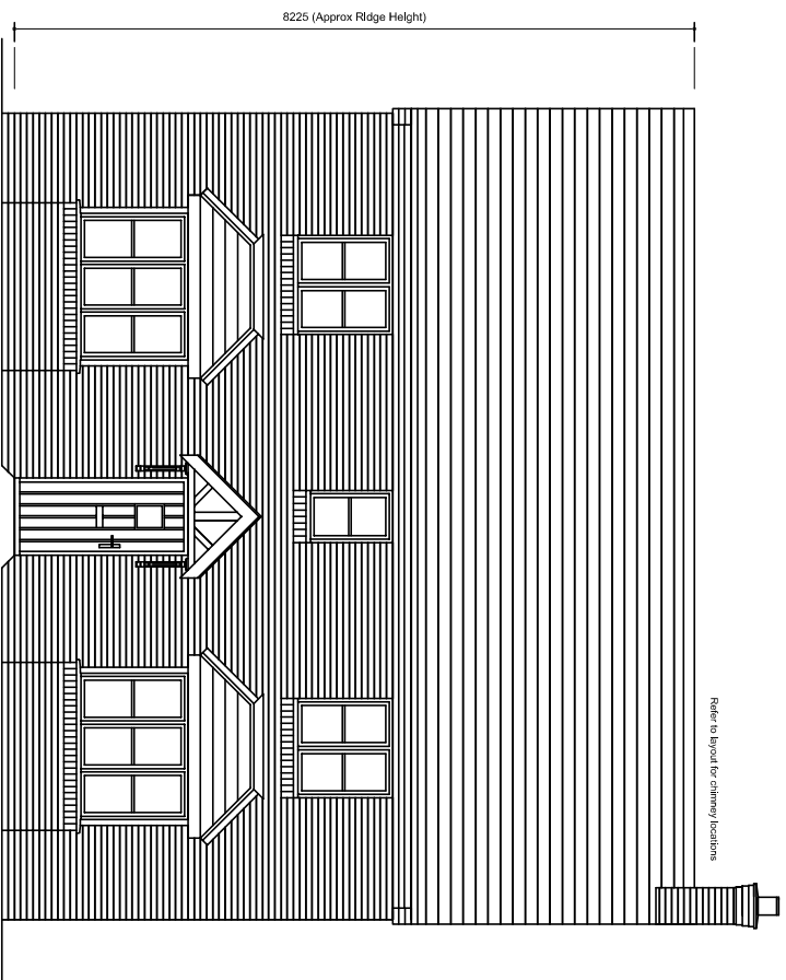
FRONT ELEVATION INFORMAL PLOT : 70,91 TYPE B : P303
