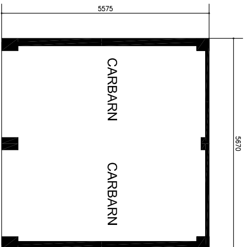
PLAN - 2 BAY
