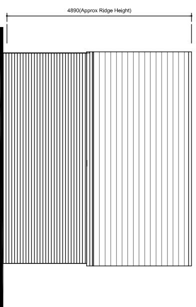
SIDE ELEVATION
