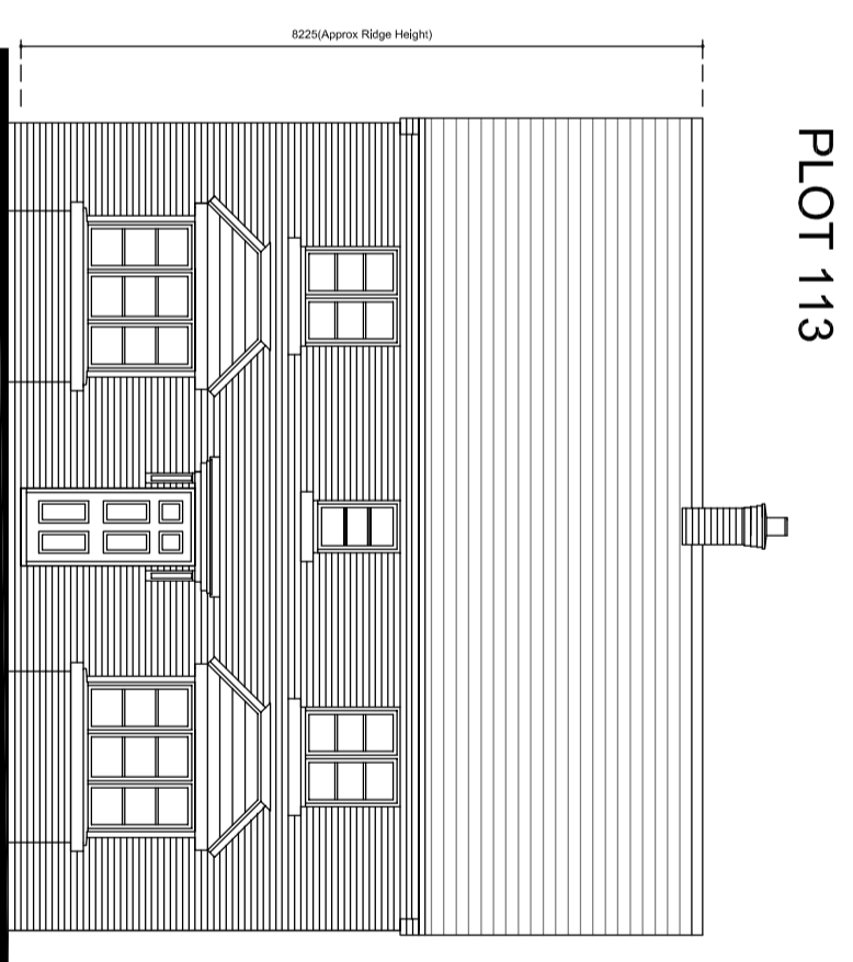
PLOT 113 FRONT ELEVATION
