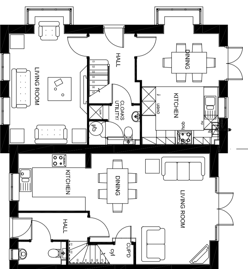
TYPE B - P303 PLOT 113 GROUND FLOOR
