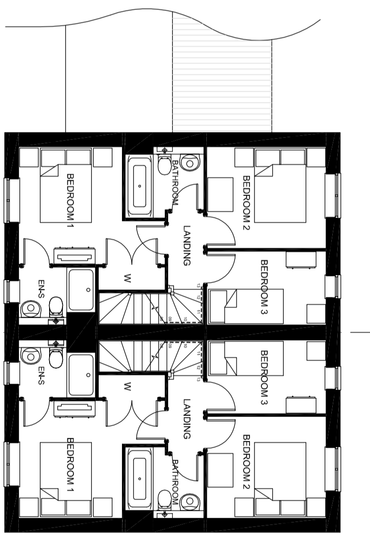
TYPE A - P302 FIRST FLOOR
