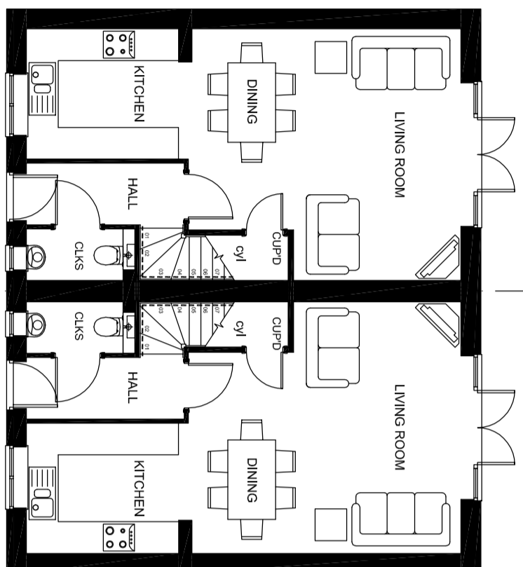
TYPE A - P302 PLOT 33 GROUND FLOOR
