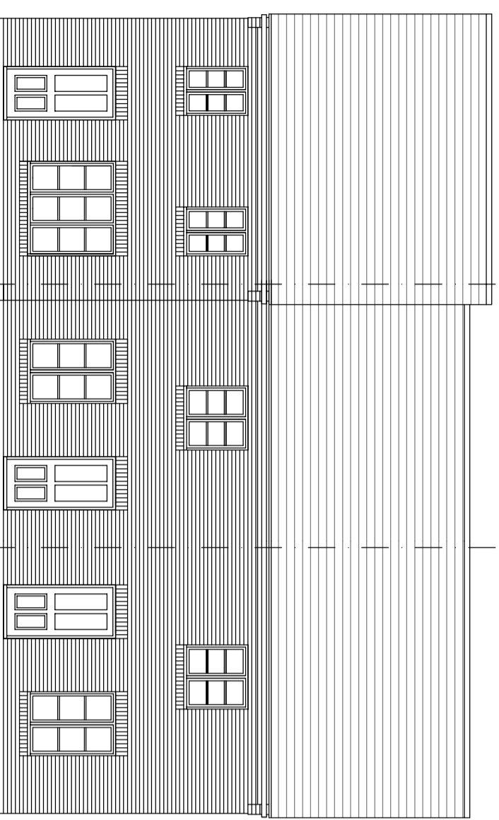
REAR ELEVATION
