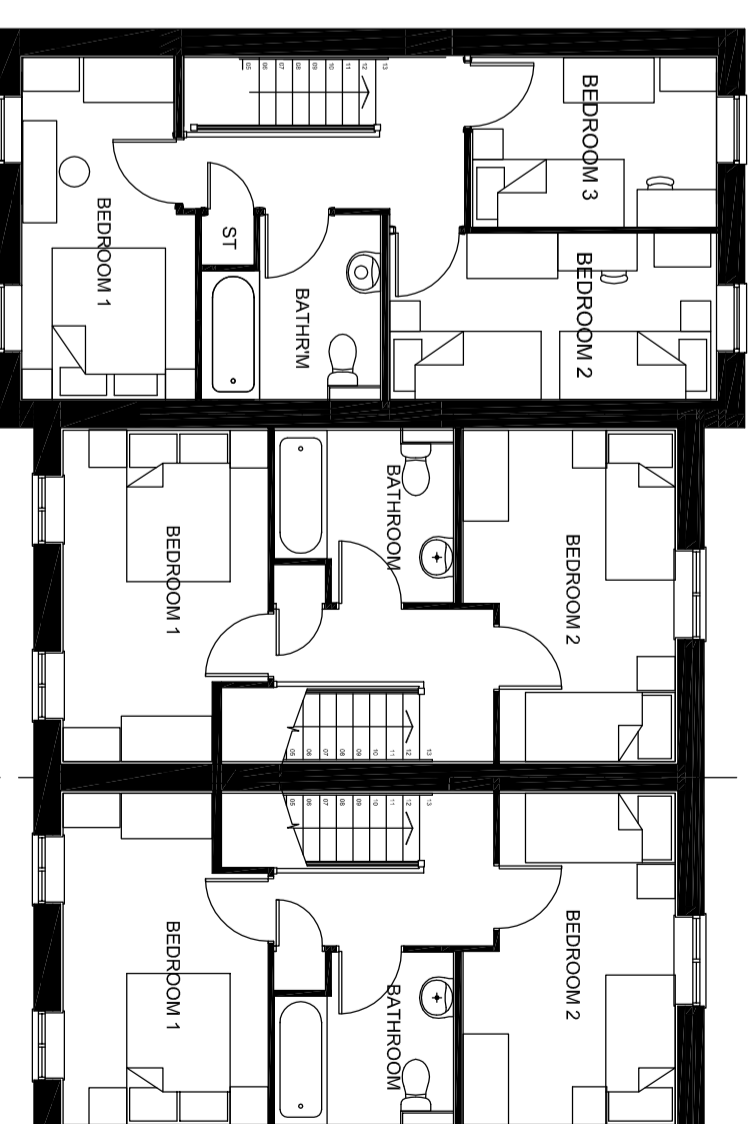
TYPE P - S351 (Rented) FIRST FLOOR
