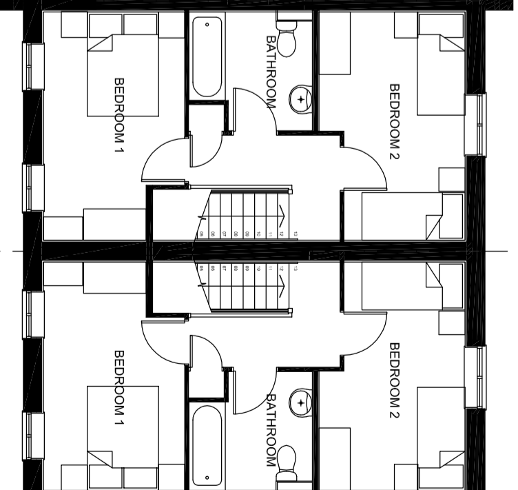
TYPE O - S241 (Rented)
