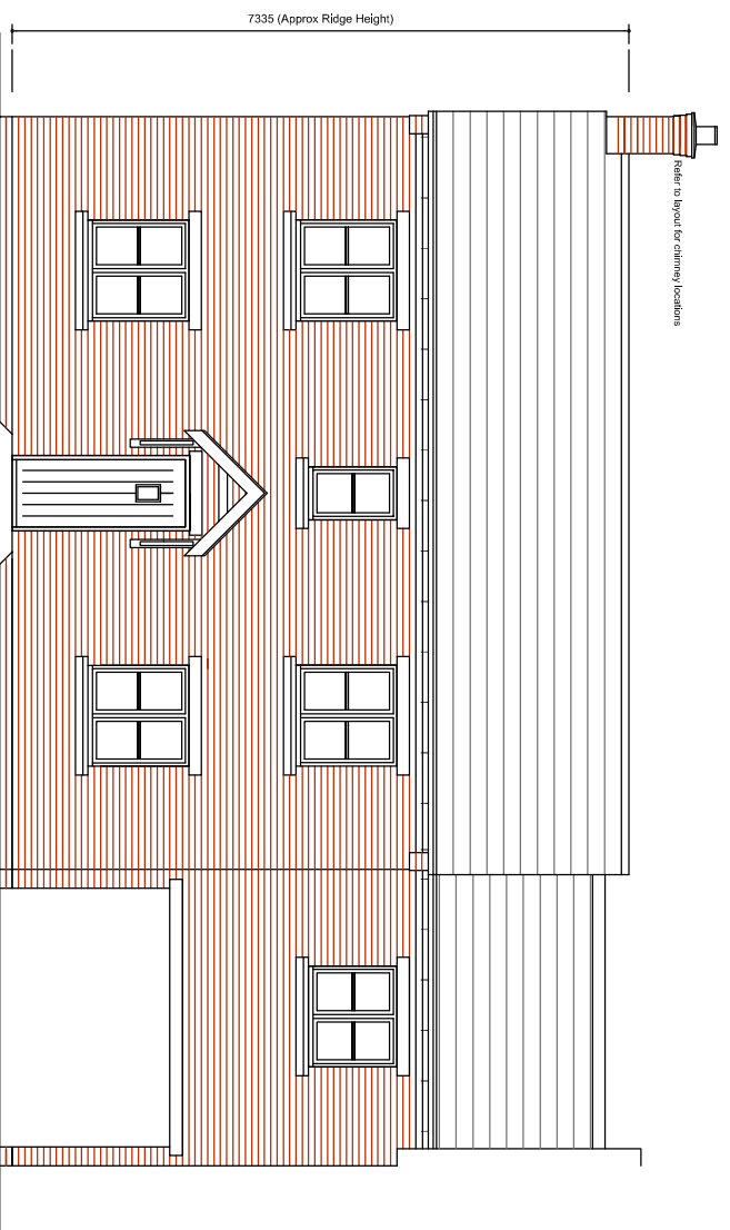
FRONT ELEVATION INFORMAL TYPE G : A548
