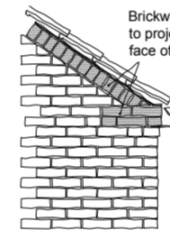
Verge detail
