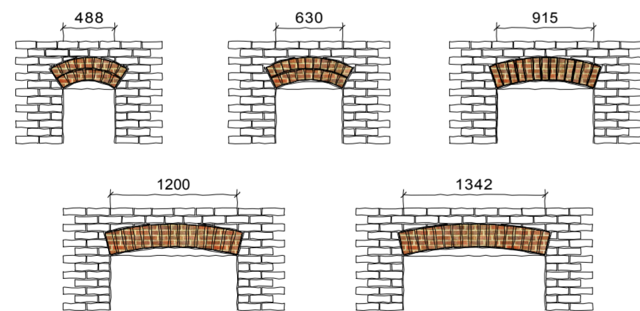
Arch Heads
