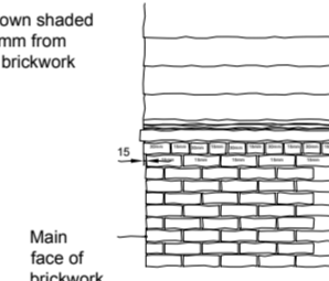
Eaves detail
