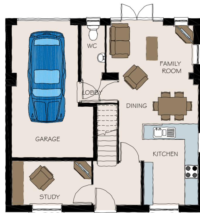
GROUND FLOOR PLAN T445---5
