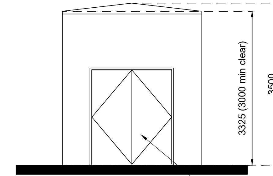
Left Elevation
