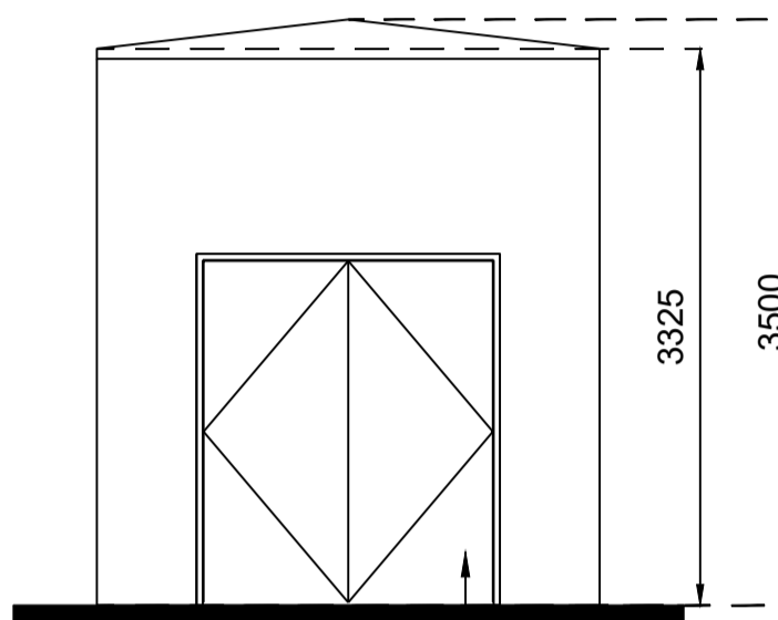
Left Elevation
