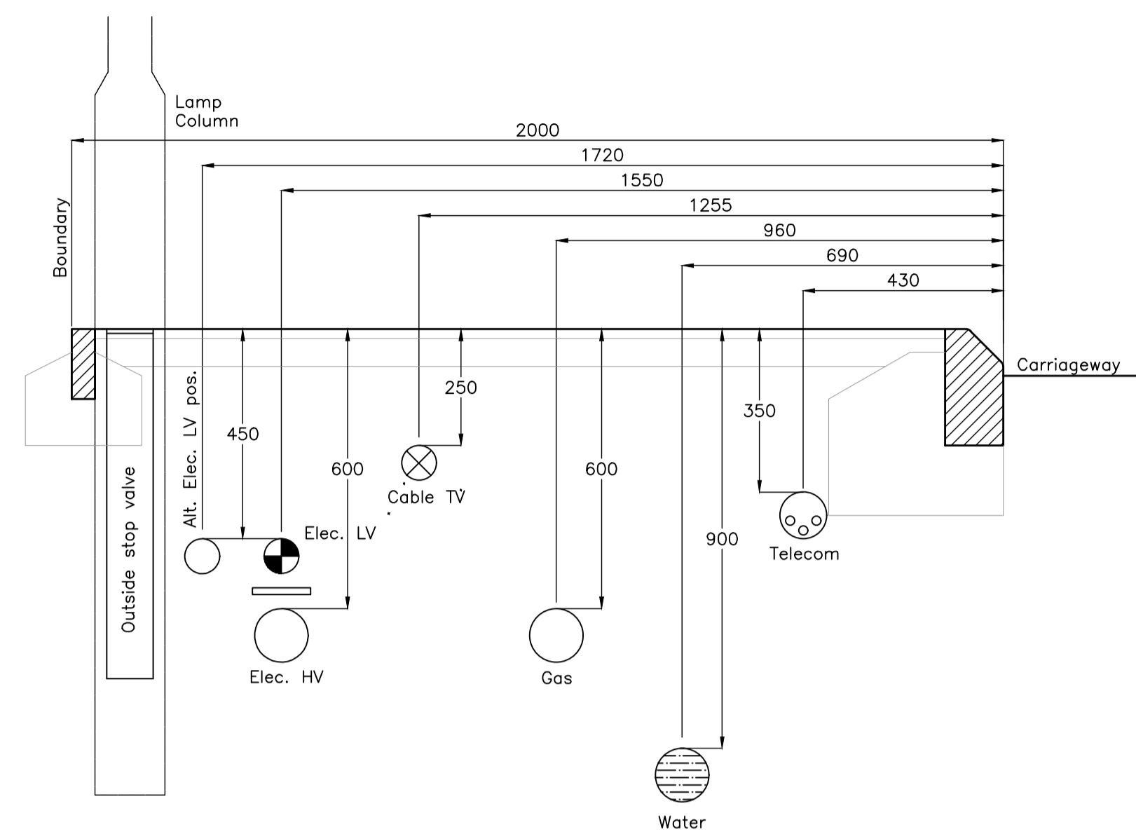
Details of Services in Footway NTS
