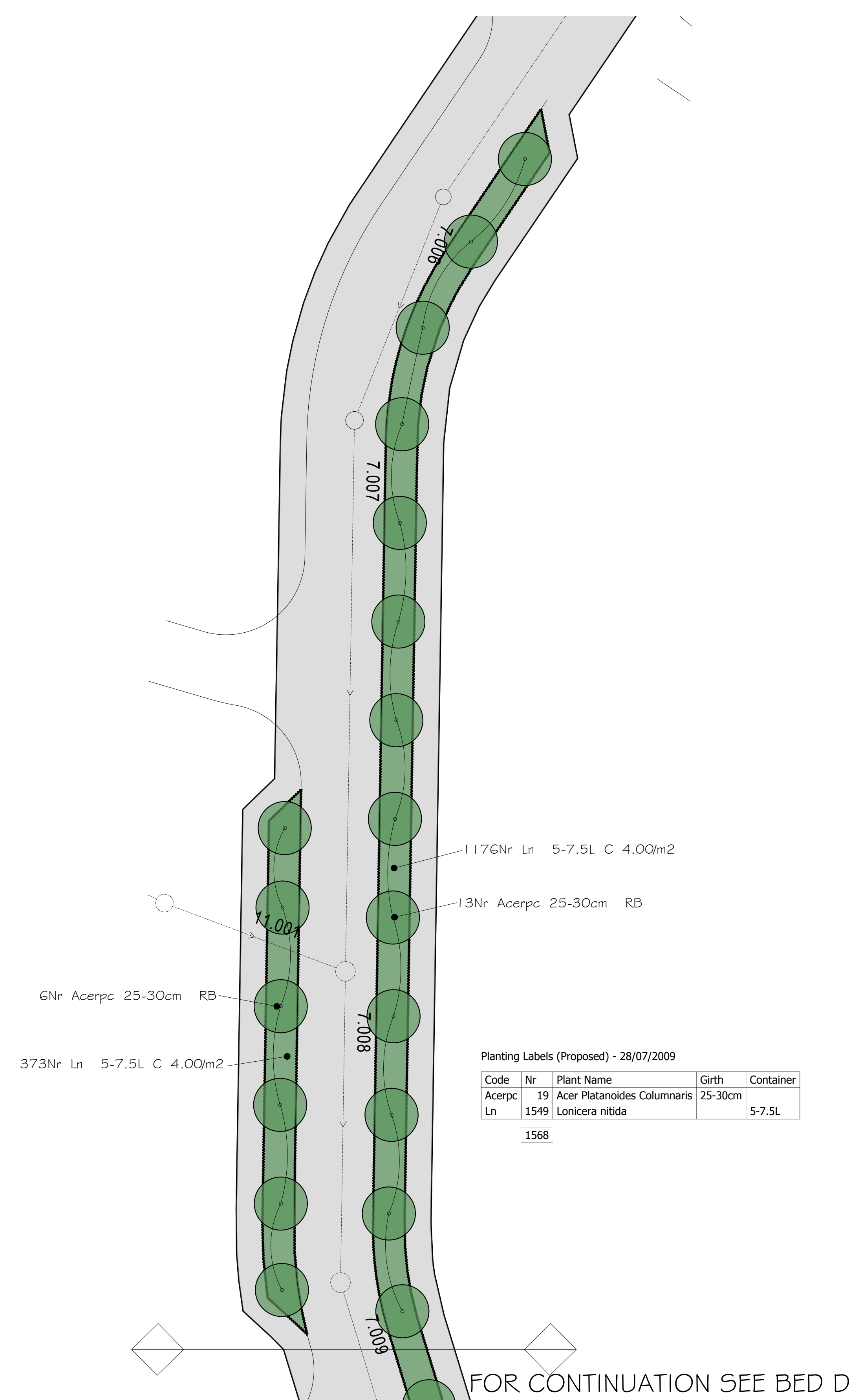
DETAIL BED C
