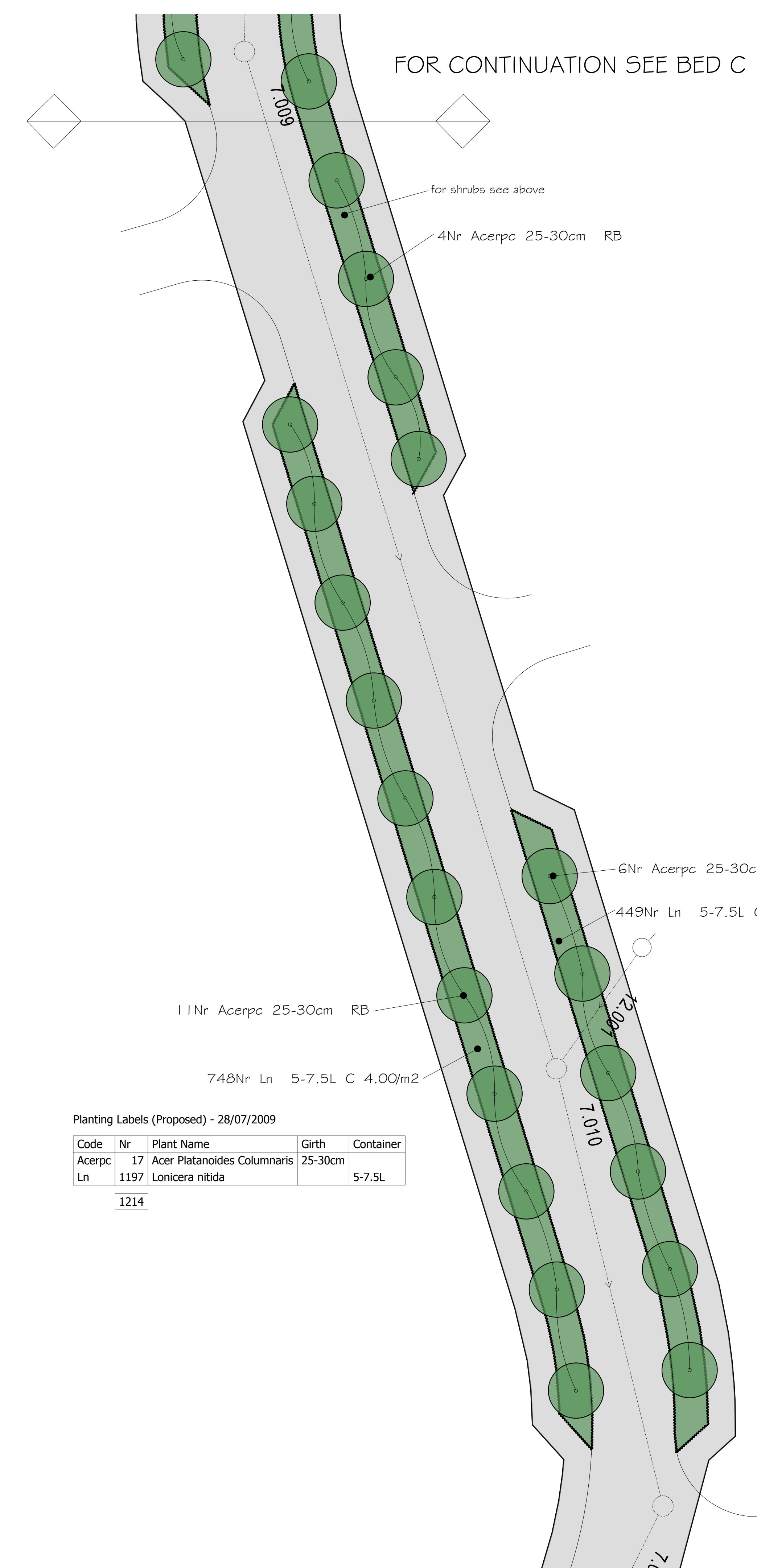
DETAIL BED D
