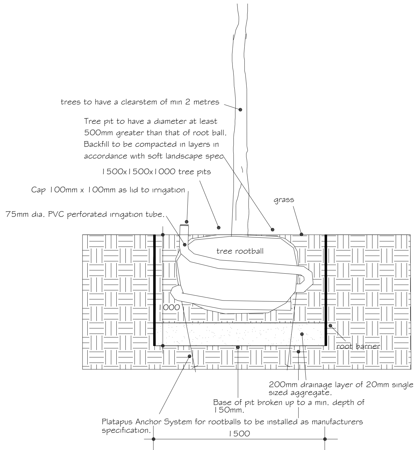
TYPICAL TREE PIT DETAIL scale 1:20
