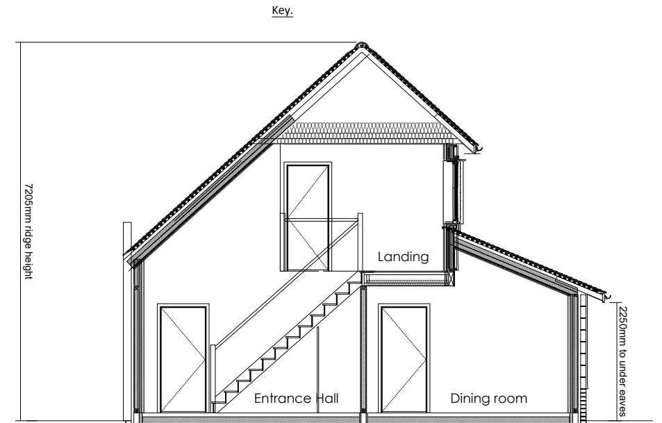
Basic section C-C
