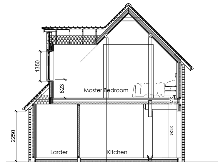
Basic section F-F
