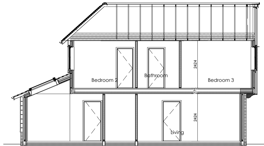
Basic section B-B
