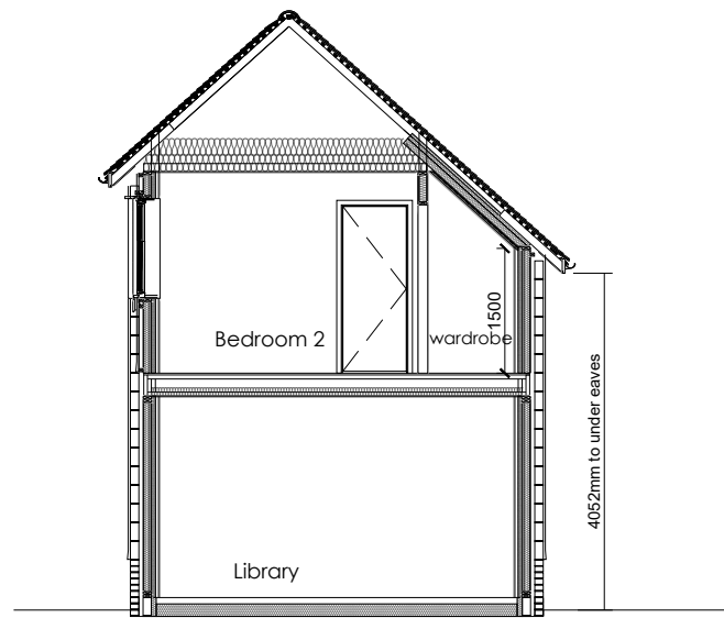
Basic section A-A
