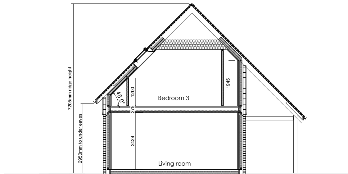
Basic section E-E
