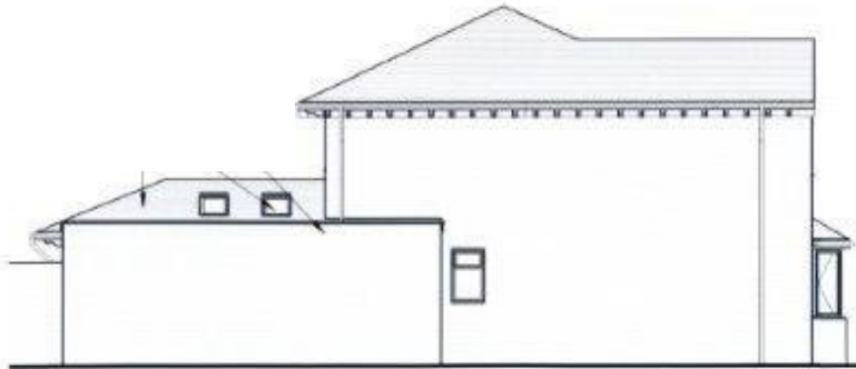
3 east elevation as proposed P104A 1:100
